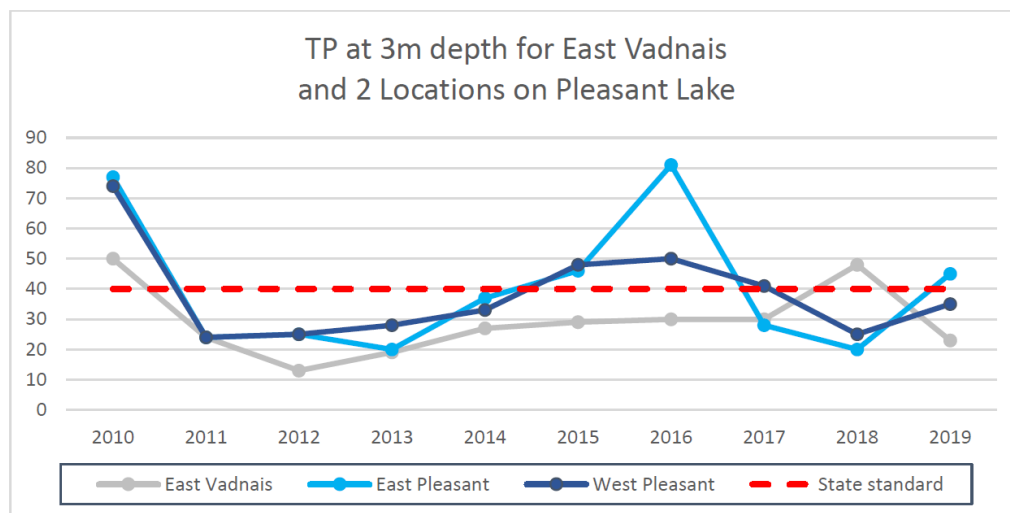
Figure 33: Total Phosphorus Comparison between East Vadnais Lake and Pleasant Lake
