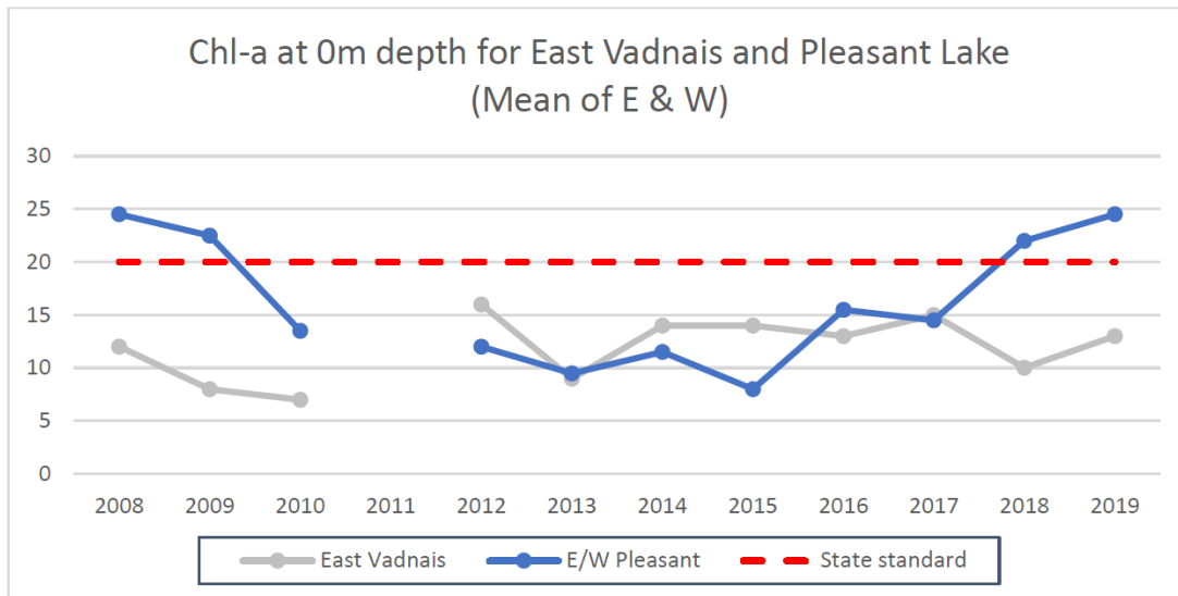
Figure 34: Chl-a in East Vadnais and Pleasant Lake
