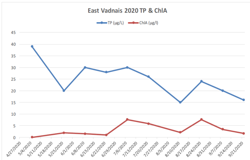
Figure 32: Water Quality Trends in East Vadnais Lake
