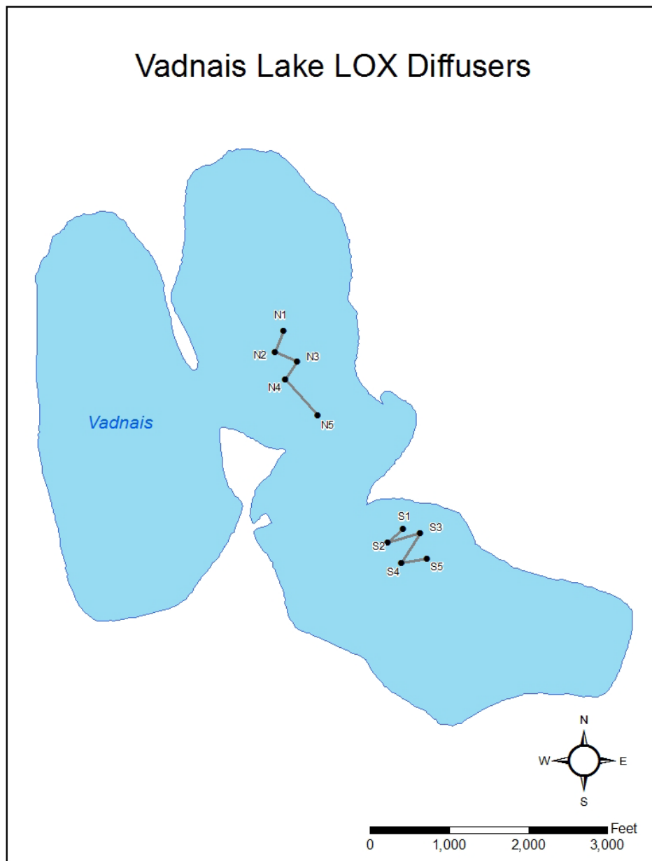
Figure 36: Liquid Oxygen Lines and Input Locations in East Vadnais Lake (contributed by SPRWS)
