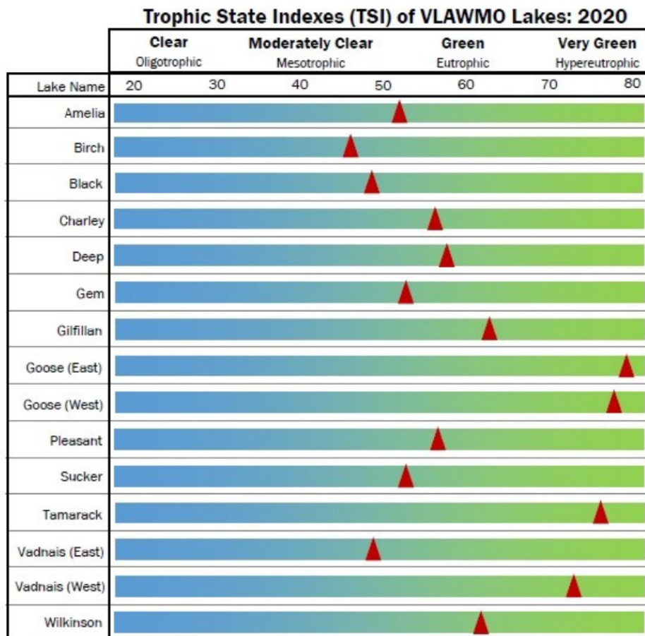
Figure 30: TSI Scores for VLAWMO Lakes
