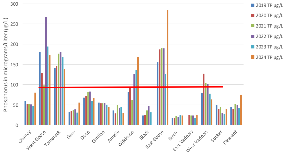
Annual Average Total Phosphorus (TP) of VLAWMO Lakes: 2019-2024
