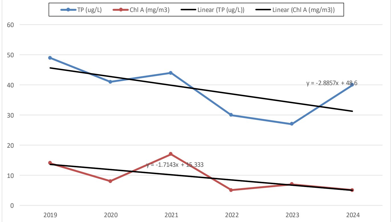
Sucker Lake Historical Avg TP & ChlA
