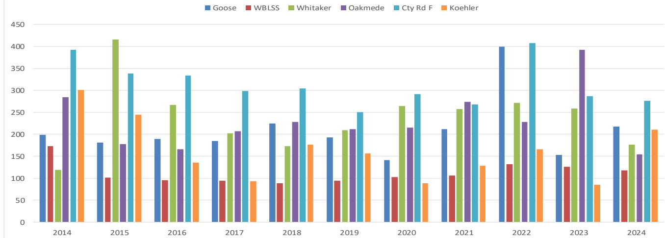
Lambert Creek Historical TP (µg/L) 2014 - 2024
