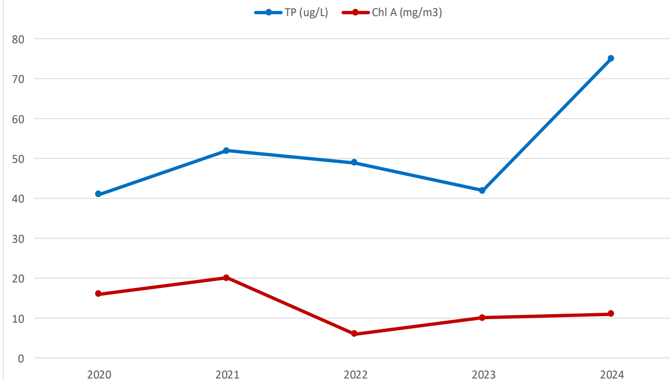
Pleasant Lake Historical Avg TP/ChlA
