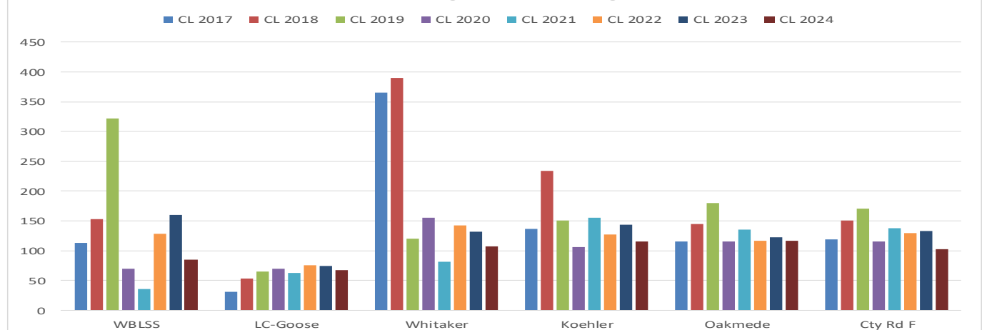
Lambert Creek Average Chloride (mg/l) 2017-2024
