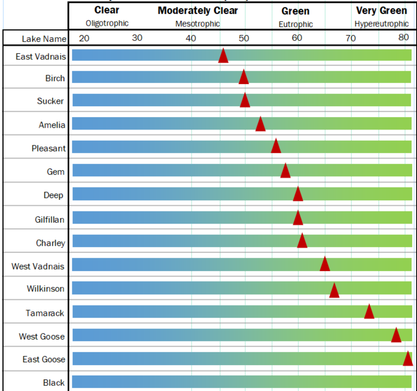
Trophic State Indexes (TSI) of VLAWMO Lakes: 2024
