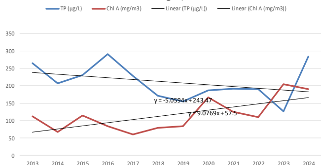
East Goose Lake Historical Avg TP/ChlA
