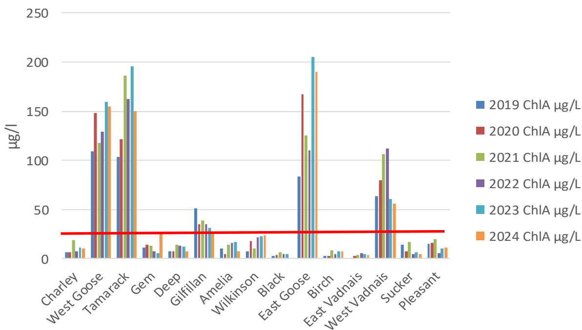
VLAWMO Lakes Average ChIA 2019-2024
