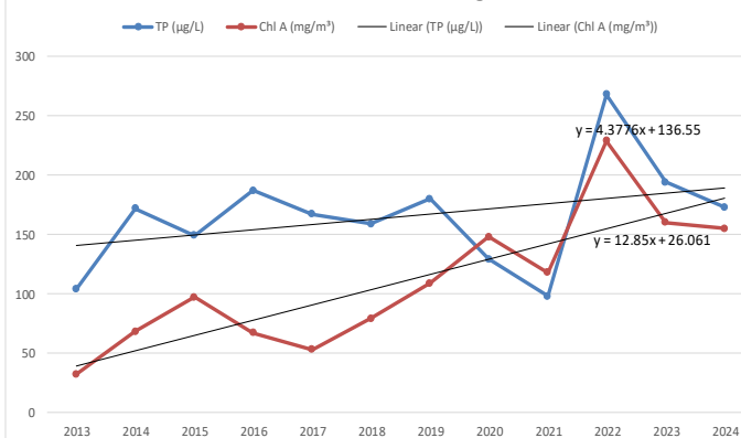
West Goose Lake Historical Avg TP/ChlA
