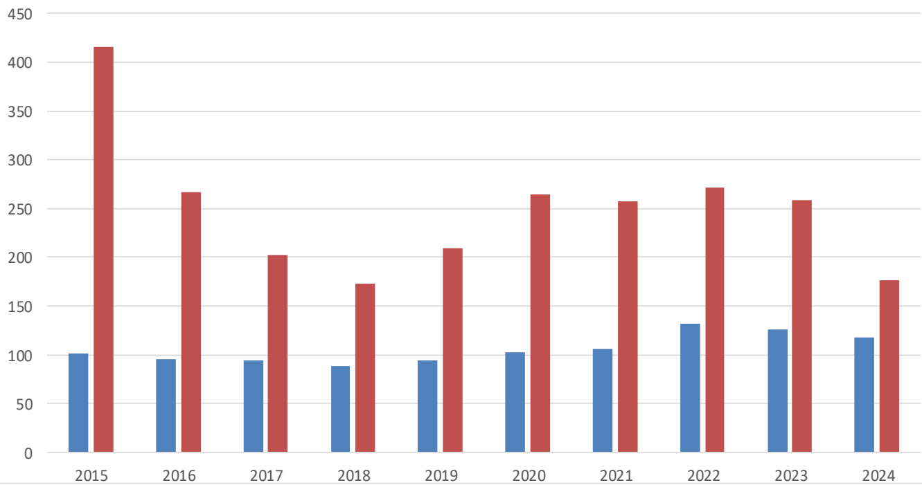
Historical TSS In & Out
