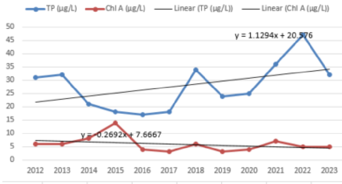
Black Lake Historical Avg TP/ChlA
