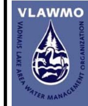
Figure 2-13 Groundwater Sensitivity
